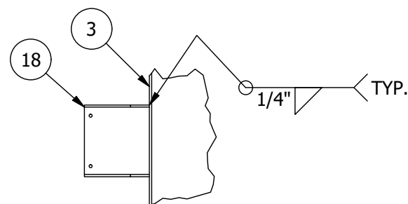
DETAIL HYD MOTOR BRKT SCALE 1 / 16
