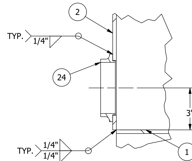
DETAIL NOZZLE SCALE 1 : 4
