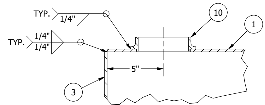
DETAIL NOZZLE SCALE 3 : 16
