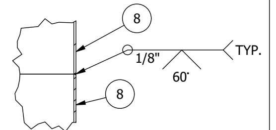
DETAIL SADDLE BUTT WELD SCALE 1 : 12
