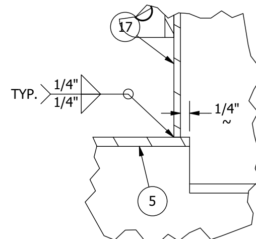
DETAIL MANWAY NECK SCALE 3 : 8
